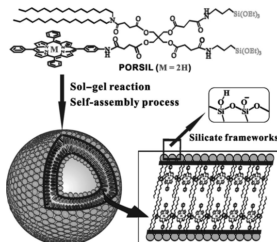
Figure 1. Formation of PBCs from a PORSIL lipid.
